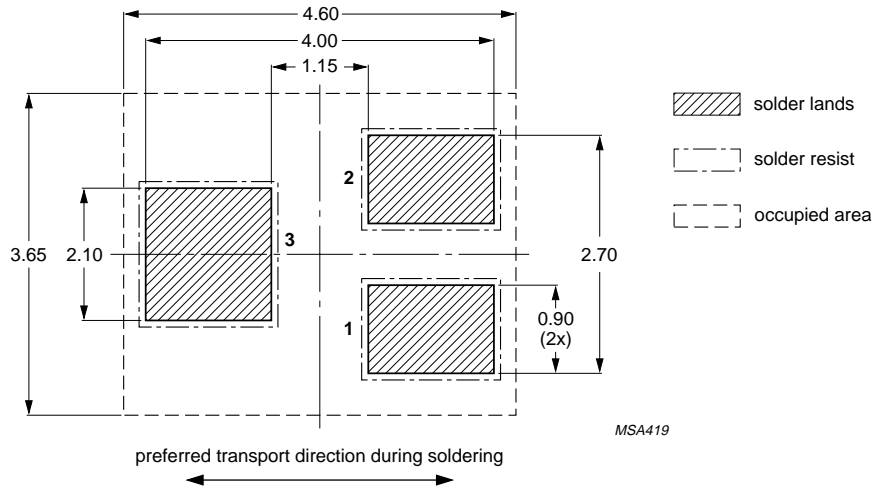
Fig 18. Wave soldering footprint SOT323 (SC-70)
